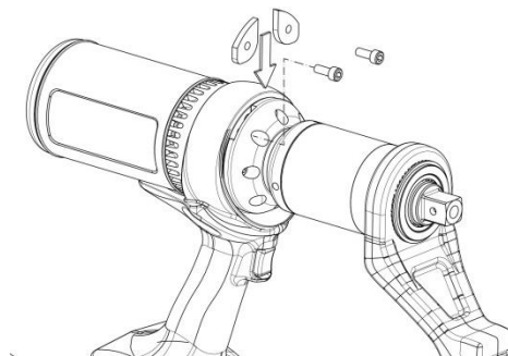
FIGURE 4 – Install infills
