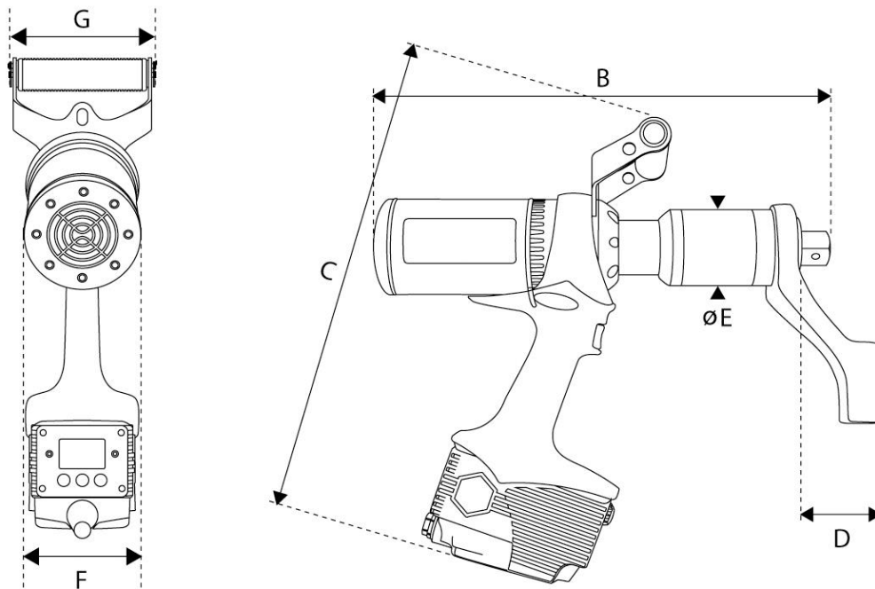
FIGURE 29 – Tool Dimensions
