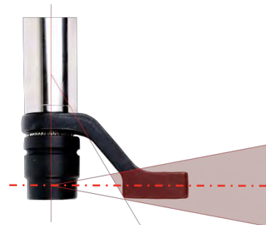
FIGURE 7 – Standard Length Socket Safe Reaction Window
